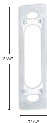
#10WDA Cover plate kit for 370 Series controls
